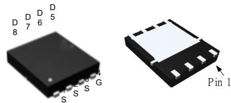
DFN5x6A-8_EP
