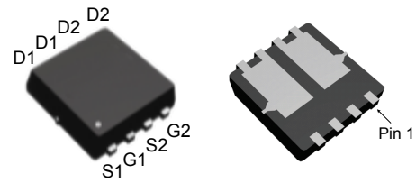
DFN3.3x3.3G-8_EP2
