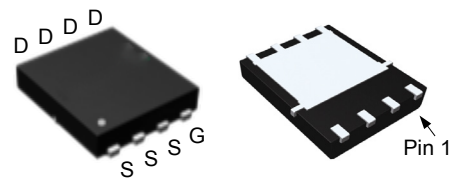
DFN5x6L-8_EP
