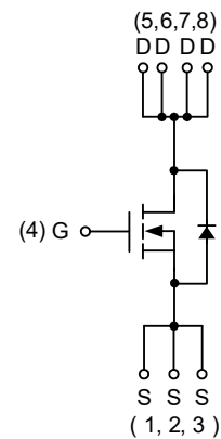
N-Channel MOSFET
