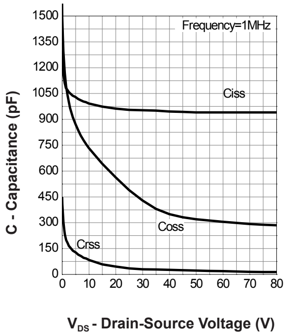
Capacitance
