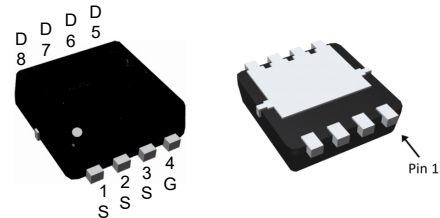
DFN3x3A-8_EP
