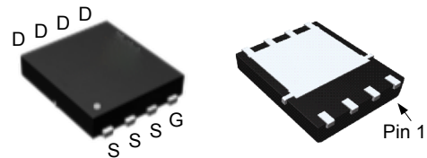
DFN5x6A-8_EP
