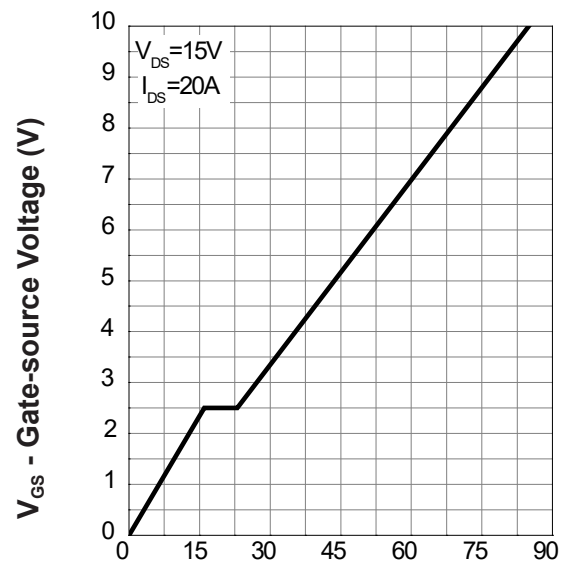
Gate Charge
