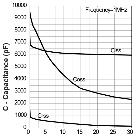
Capacitance
