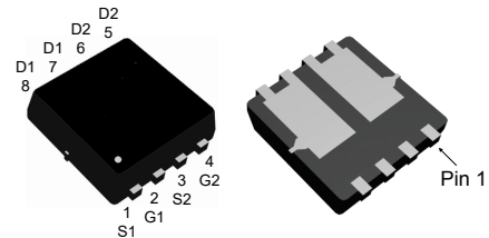
DFN3.3x3.3G-8_EP2
