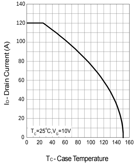
Drain Current
