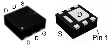
DFN2x2A-6_EP
