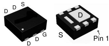
DFN2x2-6
