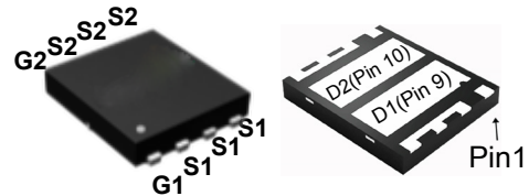
DFN5x6I-8_EP2
