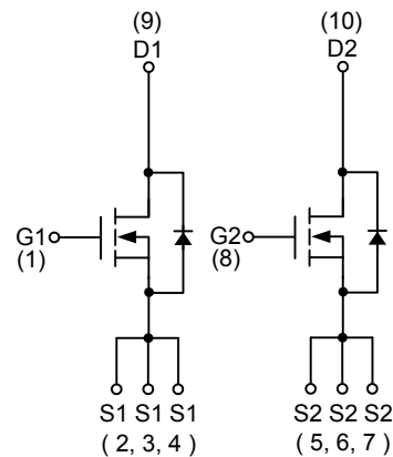
N-Channel MOSFET
