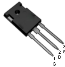
TO-247
