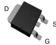
TO-252-2
