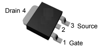
TO-252
