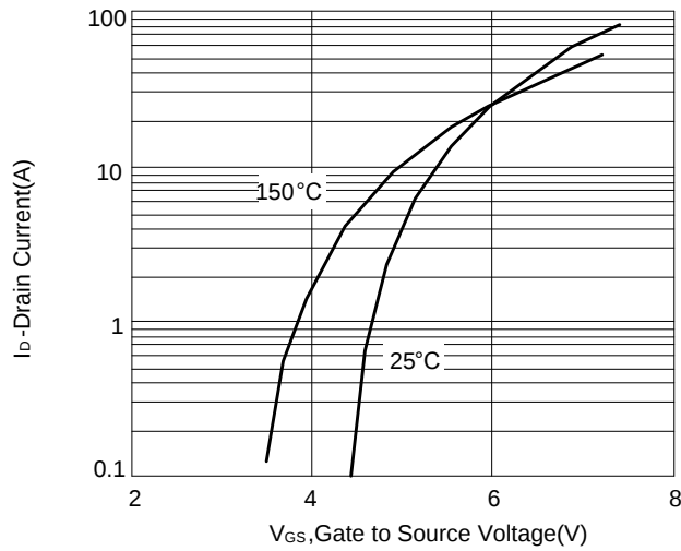
Figure 1: Transfer Characteristics
