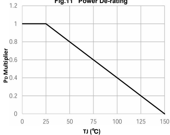
Fig.11 Power De-rating
