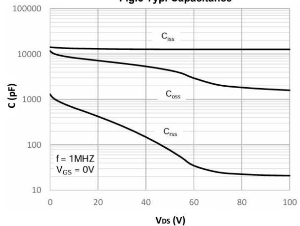
Fig.6 Typ. Capacitance
