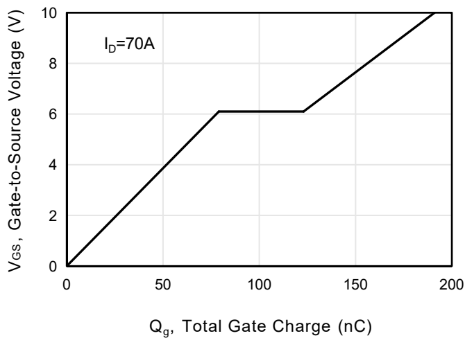
Figure 7 . Gate Charge
