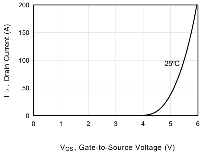
Figure 4 . Transfer Characteristics
