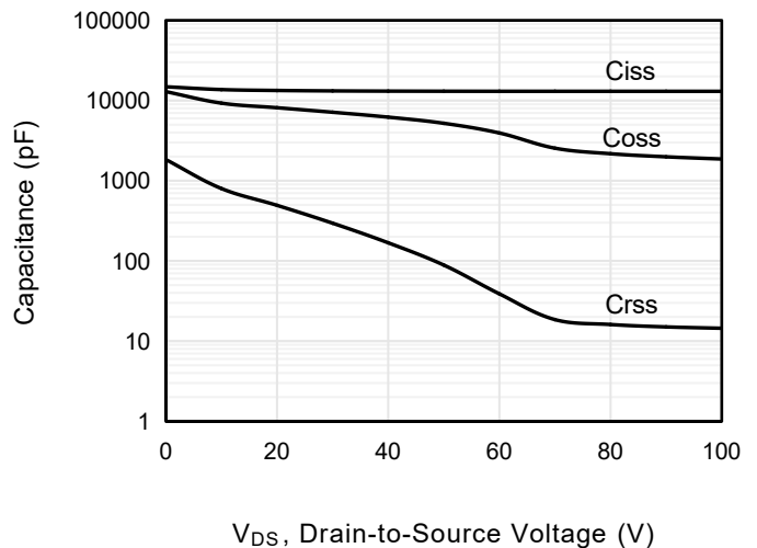
Figure 6 . Capacitance
