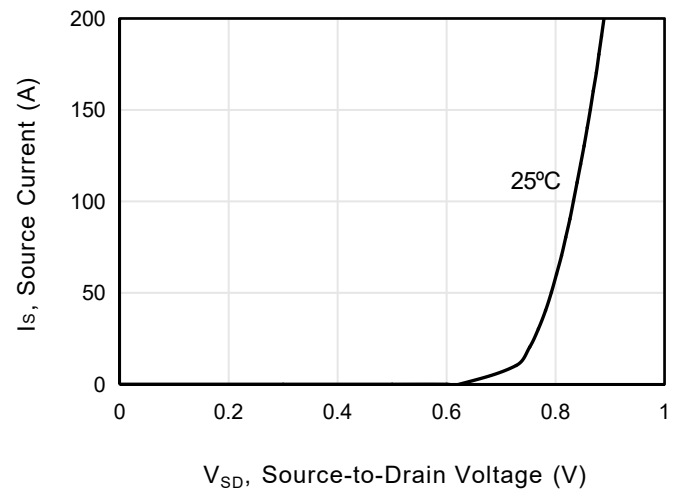
Figure 8 . Body Diode Forward Voltage
