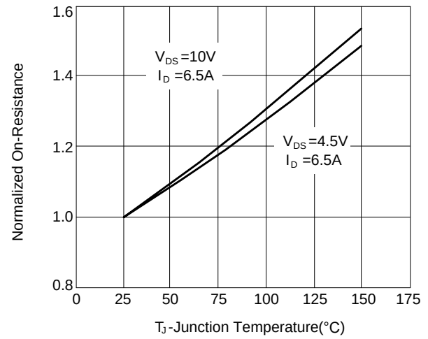
Figure 2: Rdson-Junction Temperature
