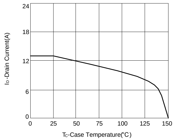
Figure 10: Current De-rating
