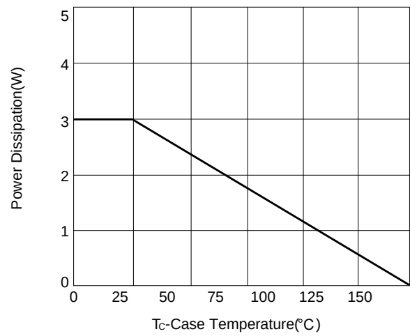
Figure 8: Power De-rating
