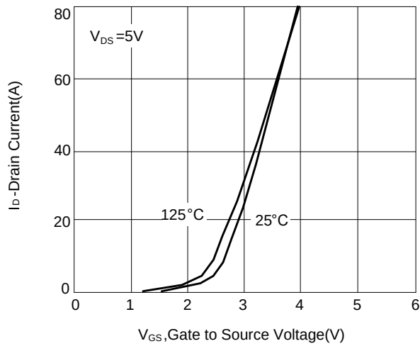
Figure 3: Transfer Characteristics
