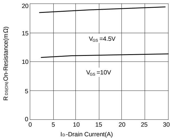
Figure 5: Rdson-Drain Current
