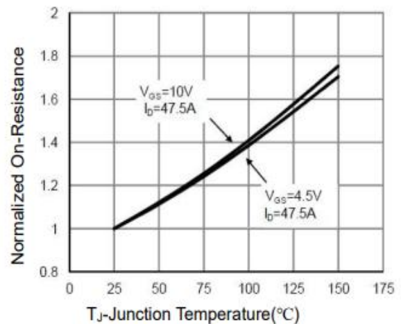
Figure 4 Rdson-Junction Temperature
