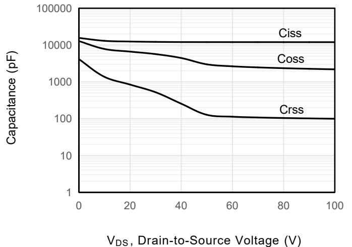
Figure 6 . Capacitance
