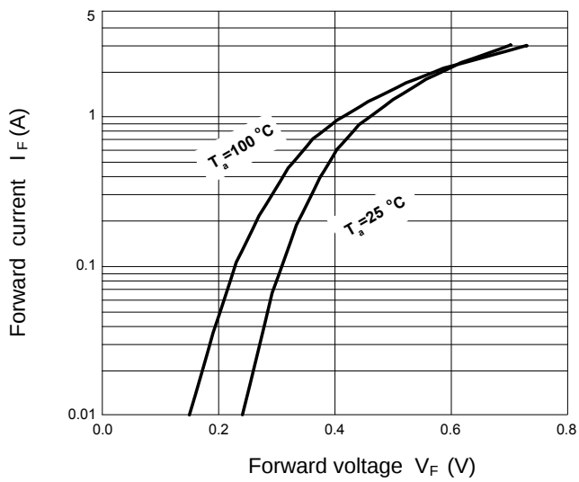
Figure 1: Forward characteristics
