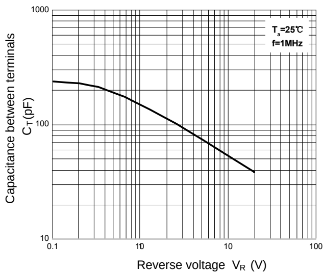
Figure 3: Capacitance characteristics
