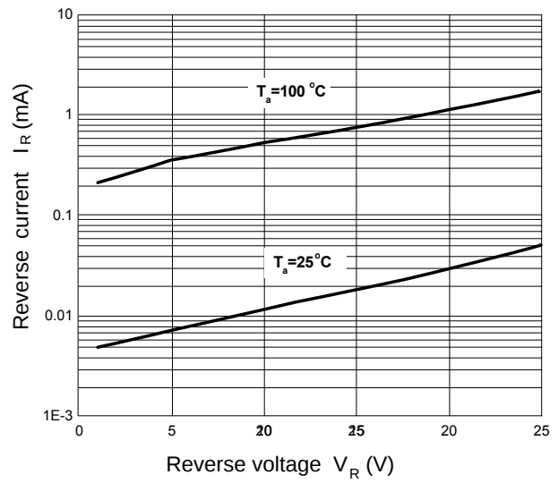
Figure 2: Reverse characteristics
